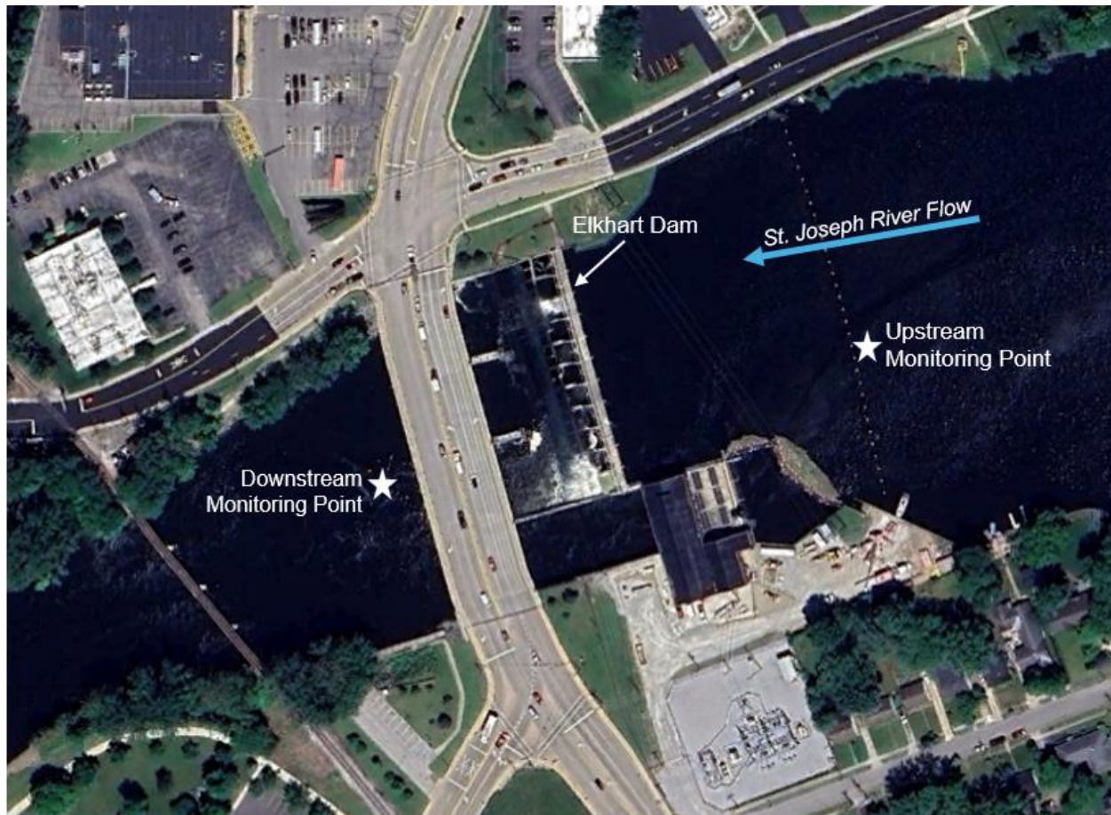
Figure 4-1. Water Quality Study Area with Proposed Monitoring Locations
